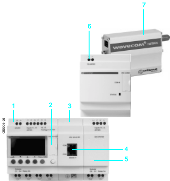
Smart relay
