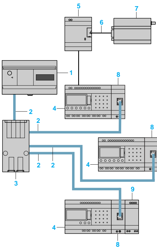
Ethernet server communication module
